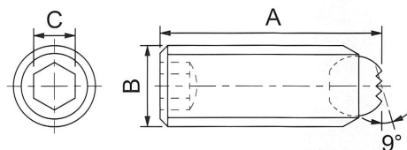
● PT16C 齒面 SERRATED END
